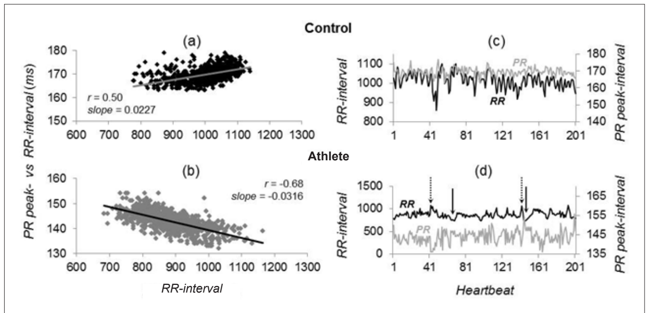
Figure 1 – Scatterplot and regression line of beat-by-beat RR-interval as a function of respective PR-peak interval of a 30 y.o. Control subject (a) and a 19 y.o. Athlete (b). Two hundred heartbeat sequences of respective RR- and PR-peak intervals series are shown in (c) and (d). In (a), PR-peak interval increases as RR interval increases (positive slope: 0.0227; r = 0.50 ; p < 0.01 ), clearly observed in (c) (spontaneous concordant condition). Conversely, in (b), PR-peak interval decreases as RR interval increases (negative slope: -0.0316; r = -0.68 ; p < 0.01 ). In (d), note periods of reciprocal variation in RR- and PR-peak intervals (spontaneous discordant conduction): PR-peak interval shortens as RR-interval increases (dotted arrow) and PR-peak interval increases as RR-interval shortens (decremental conduction, solid arrow) (see text for details).
