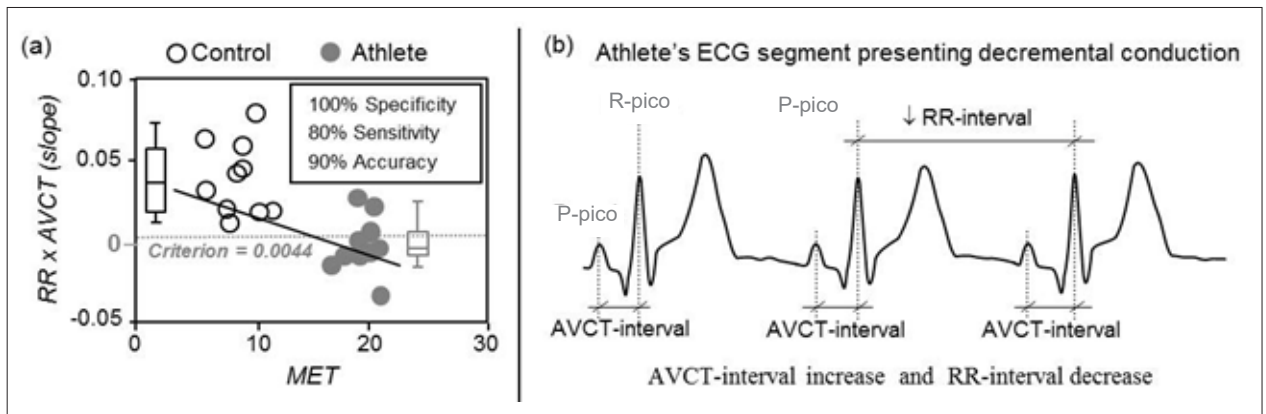
Figure 2 – (a) Regression line slope values of pooled AVCT vs. mean RR-intervals (RR-AVCTslope) as a function of VO_2 consumption expressed as maximal metabolic equivalent (MET) achieved during stress test and respective boxplot. Note that RR-AVCTslope tends to be more negative as physical conditioning status increases (grey dots), when compared to sedentary individuals (white dots). Box-plots showing median, interquartile range and 95% confidence intervals are shown in the vicinity of the respective group points. Specificity, sensitivity and accuracy values were computed utilizing RR-AVCTslope = 0.0044 as a cut-off criterion. (b) Illustration of 19 y.o. Athlete's ECG segment depicting a sequence of normal sinus beats showing AVCT lengthening as RR-interval decreases, indicating AV decremental conduction. Note P-wave and R wave peaks taken as the fiducial points for assessment of the PR-peak interval. AVCT was assessed as PR peak interval. AVCT – atrioventricular conduction time (see text for details).
